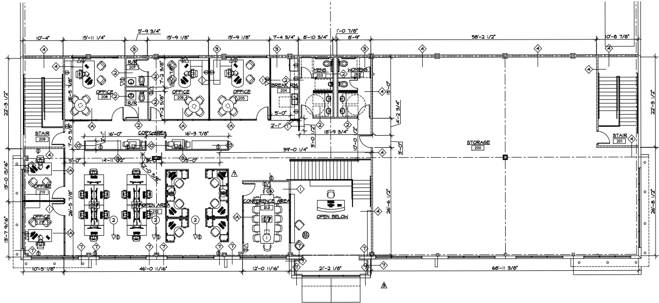
SECOND FLOOR DIMENSION FLOOR PLAN 1/8" = 1'-0" 4
