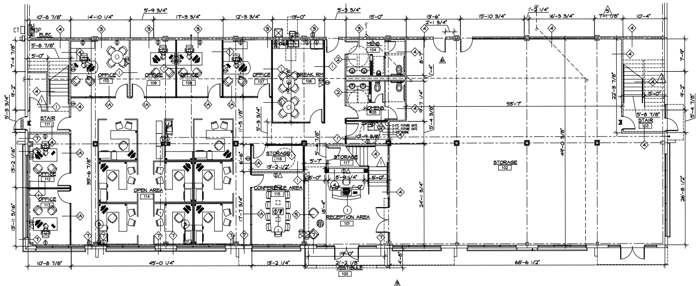
FIRST FLOOR DIMENSION FLOOR PLAN 1/8" = 1'-0" 3
