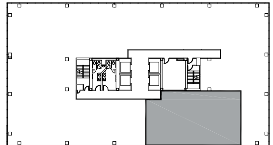
LOCATION PLAN
