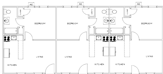
CURRENT CONFIGURATION
