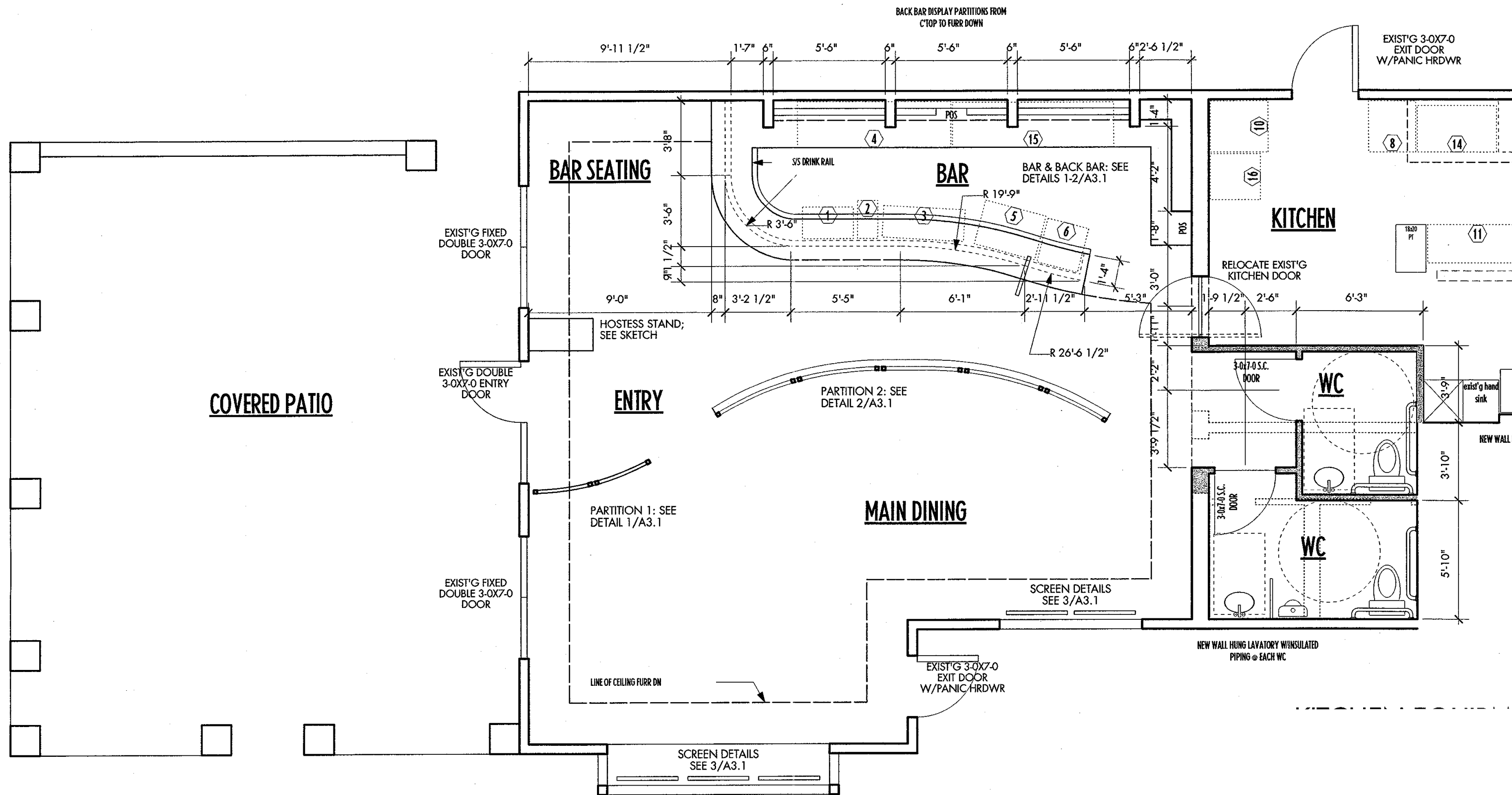
1 FLOOR PLAN A1.1 Scale: 1/4" = 1'-0"
