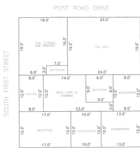
INTERIOR FLOOR PLAN LAYOUT SHEET
