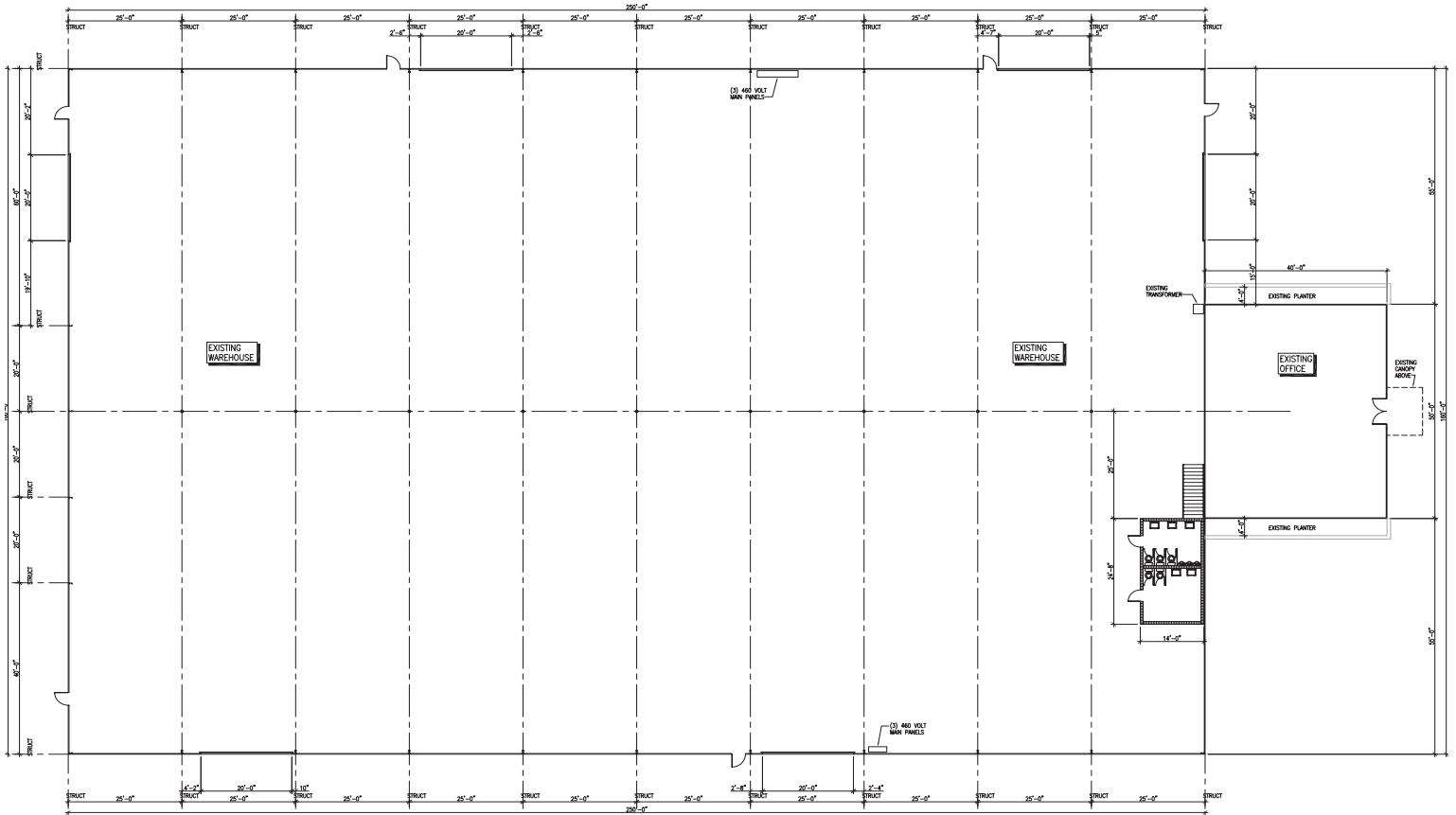
1 EXISTING FLOORPLAN 0 10'-0" 20'-0" 30'-0"
