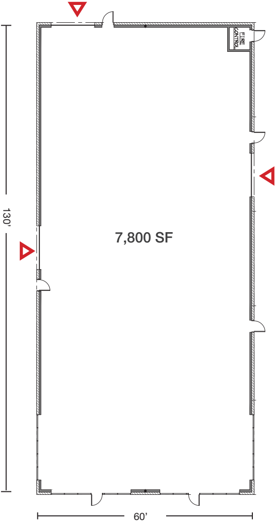
BUILDING PLAN
