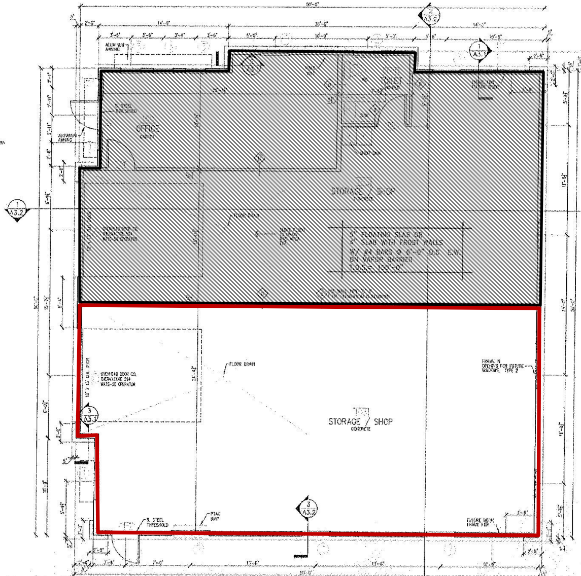
1 PROPOSED MAIN FLOOR PLAN SCALE: 1/4" = 1'-0"
