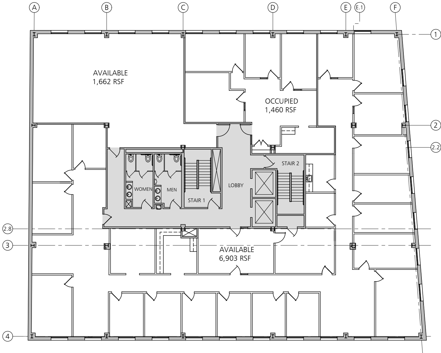
○ 2ND FLOOR PLAN SCALE: 1/16" = 1'-0" 4/15/2022
