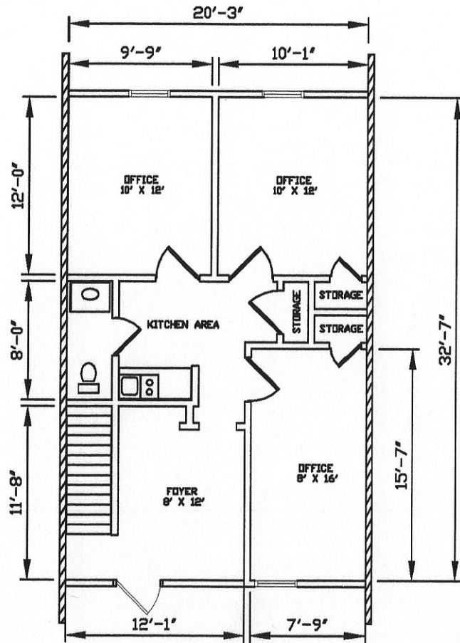
UNIT C-3 FIRST FLOOR FIRST FLOOR SQ. FOOTAGE = 659 SF.
