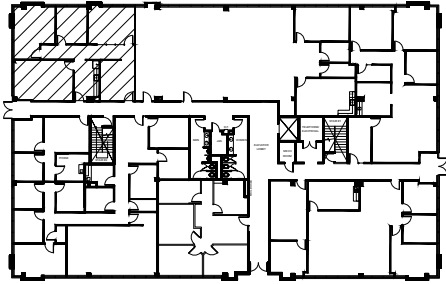
KEYPLAN - 1ST FLOOR
