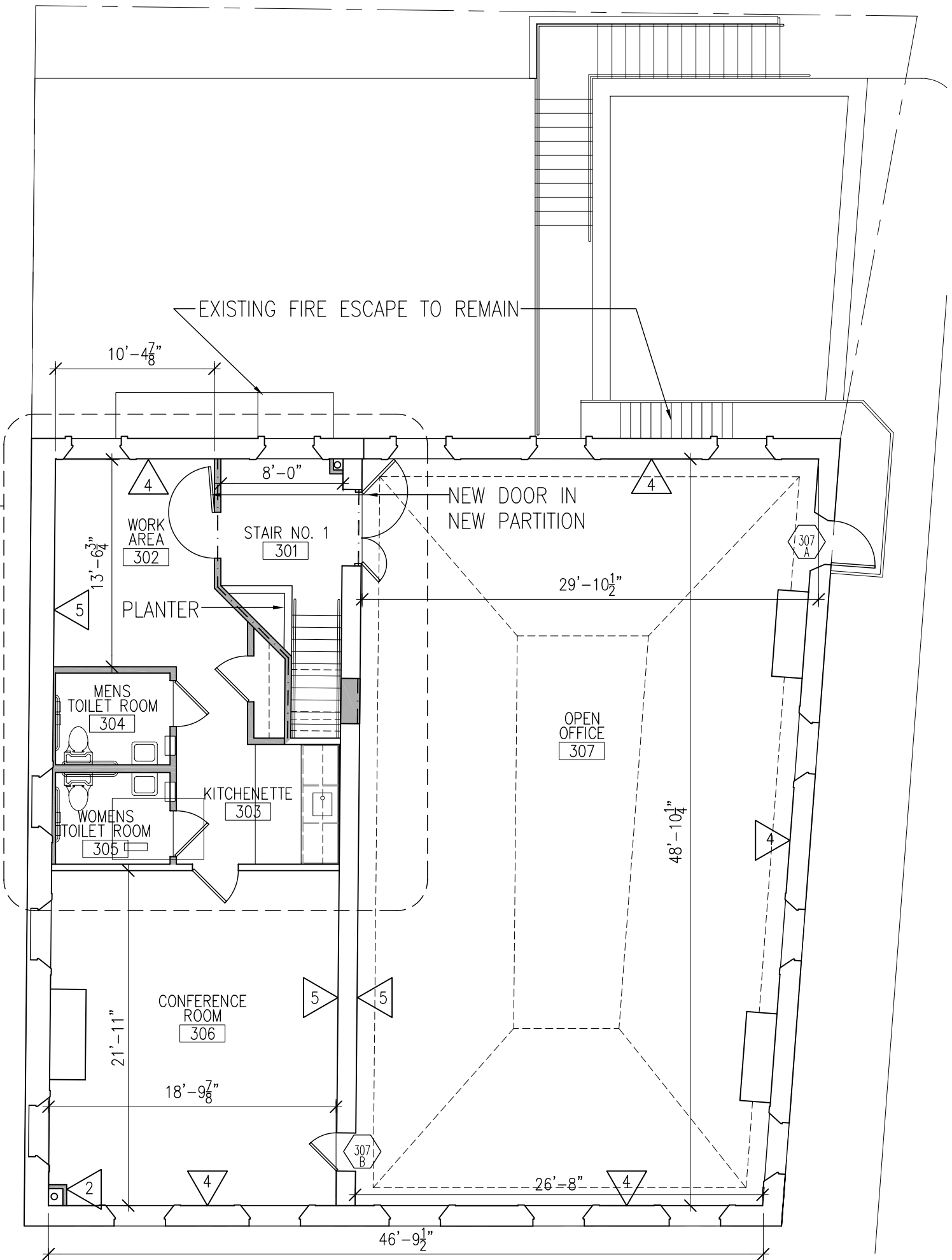
3 THIRD FLOOR PLAN 1/8" = 1'-0"
