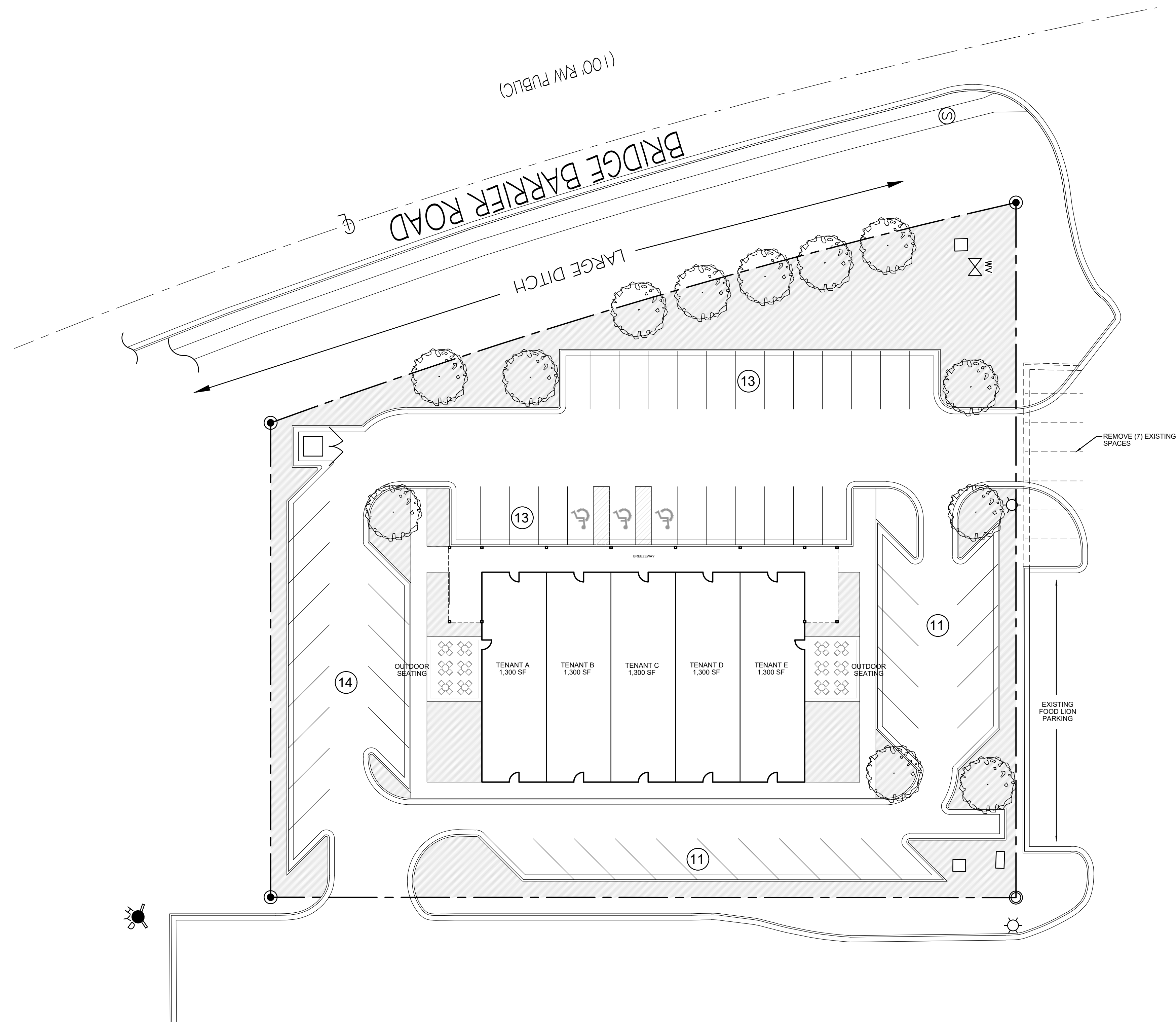
1 CONCEPT PLAN A101 SCALE: 1" = 20'-0"
