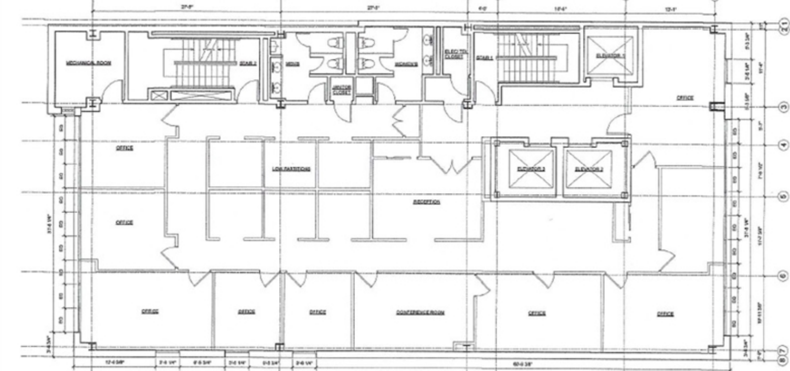
Entire 5 th Floor Plan Existing Conditions
