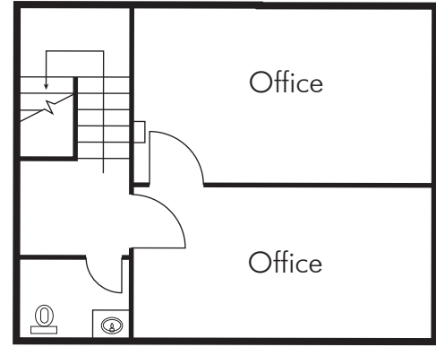
MEZZANINE
