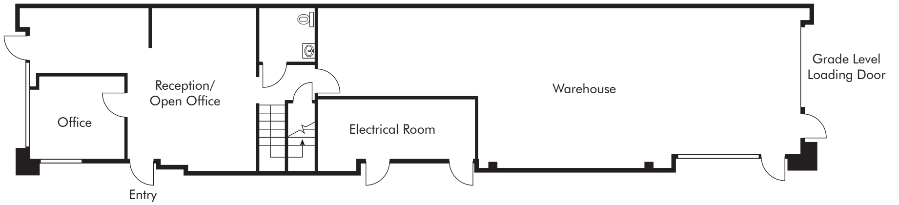
FIRST FLOOR
