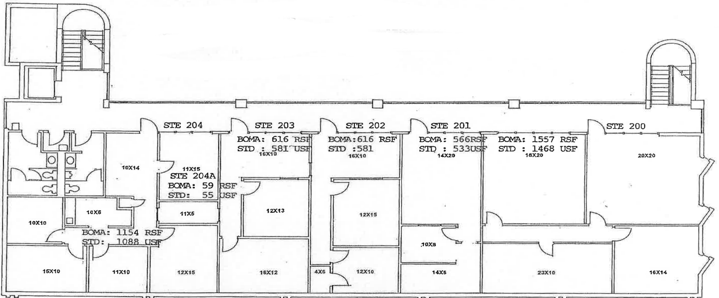
FLOOR PLAN
