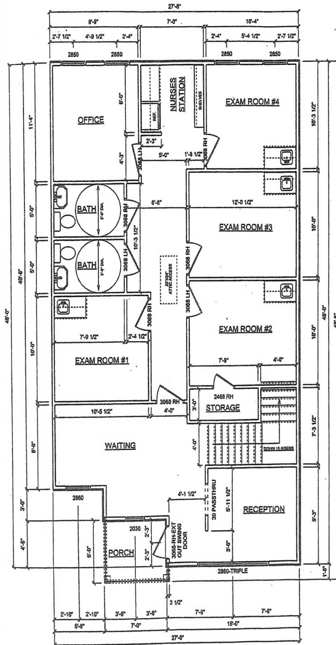
FLOOR PLAN UNIT 902
