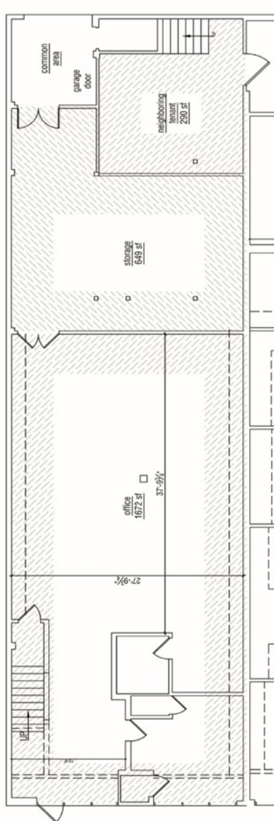
1st Floor Plan
