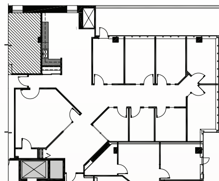
8TH FLOOR | SUITE 800 - 2,754 SF
