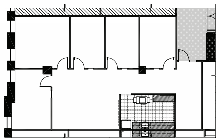
3RD FLOOR | SUITE 300 - 2,043 SF
