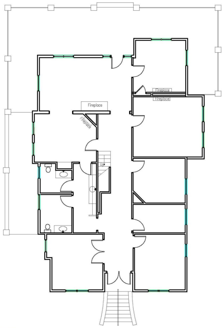
First Floor
