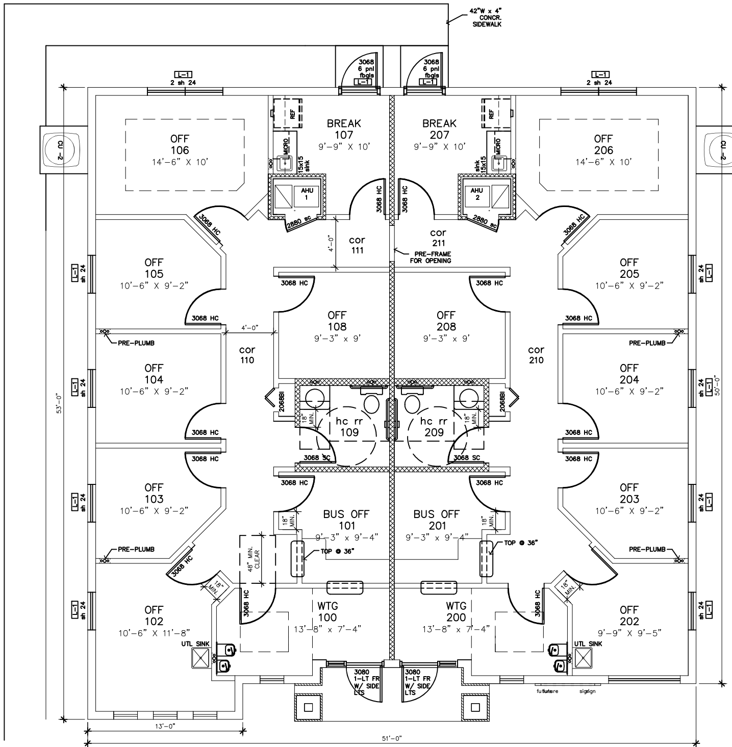
CYPRESS BEND #3 - 2570 SF Prelim #1 WATERFORD CONSTRUCTION - 6.30.22
