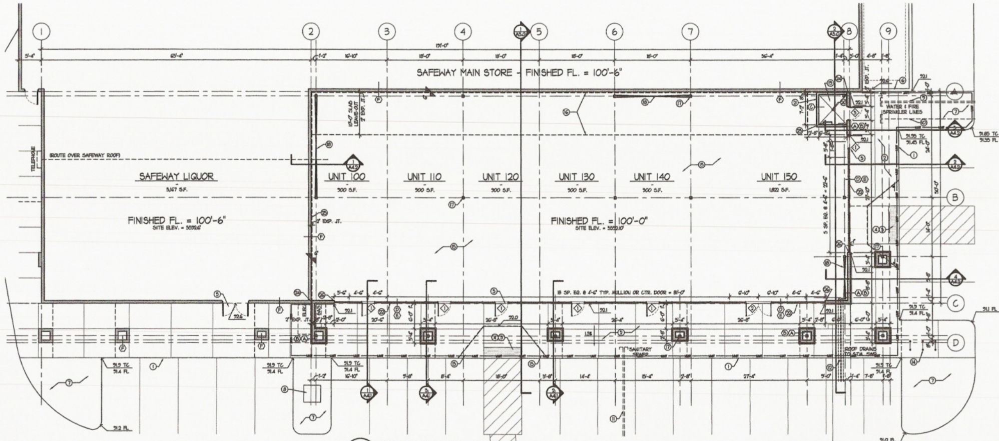
1 FLOOR PLAN SCALE 1/8" = 1'-0" NORTH
