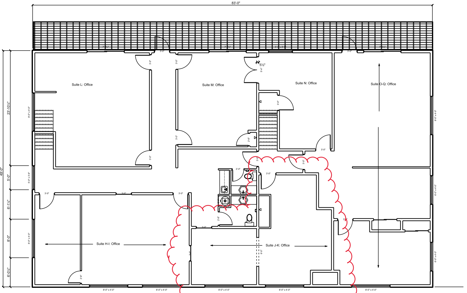
Saratoga Gateway Building 12333 Saratoga-Sunnyvale Road Second Floor Suites H - Q Existing Floor Plan. Suite Area 3,349 sft
