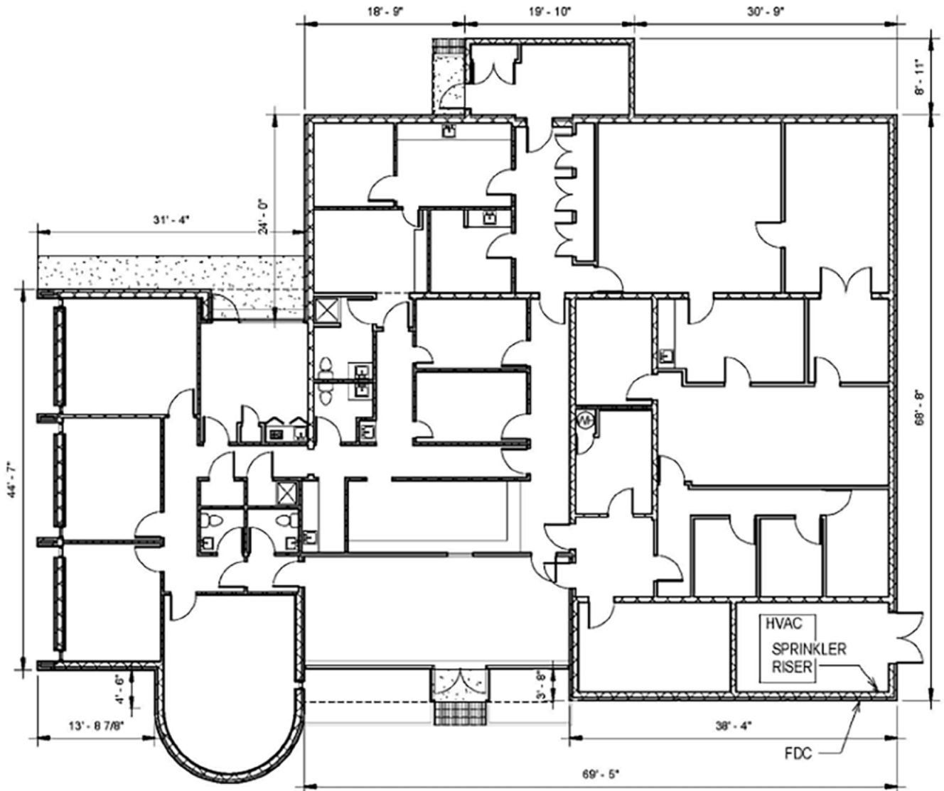
1 Existing Plan Layout A-1.01 3/32" = 1'-0"
