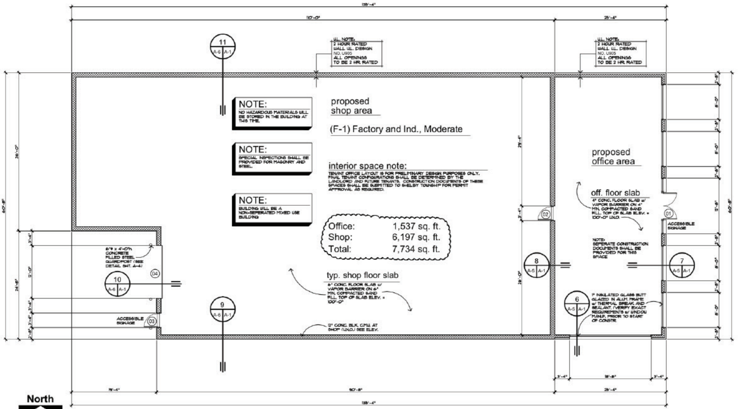
floor plan - building I
