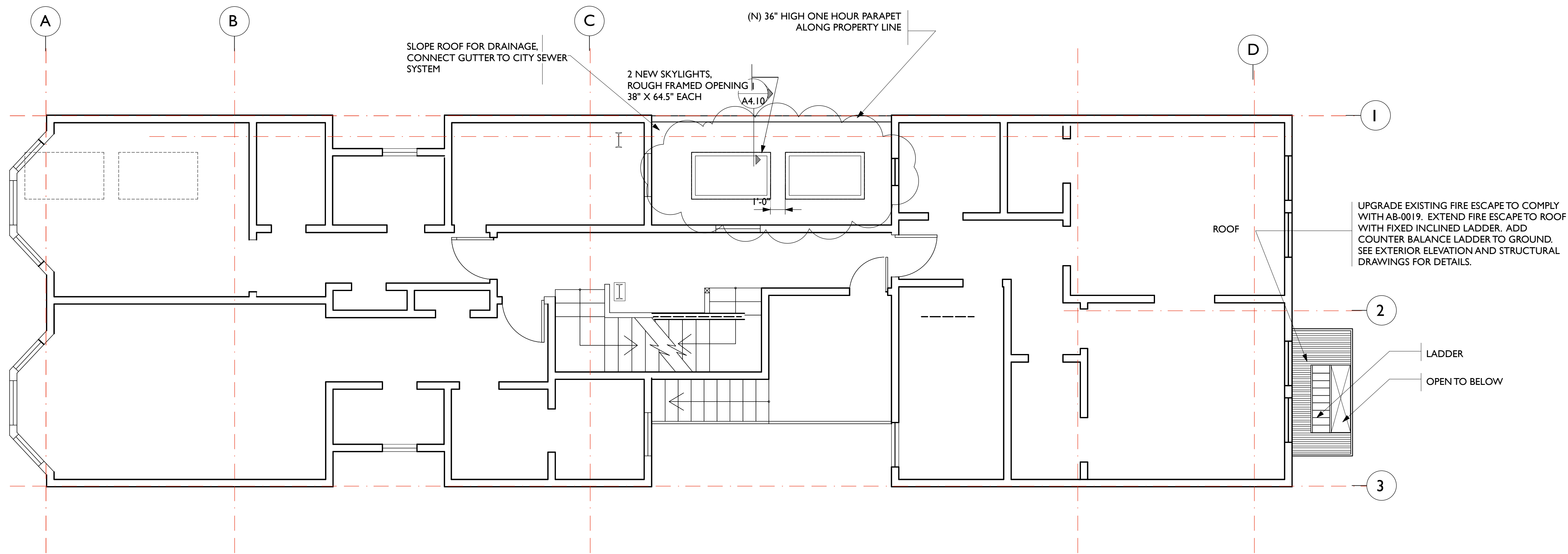
1 PROPOSED UPPER FLOOR PLAN Scale: 1/4" = 1'-0"
