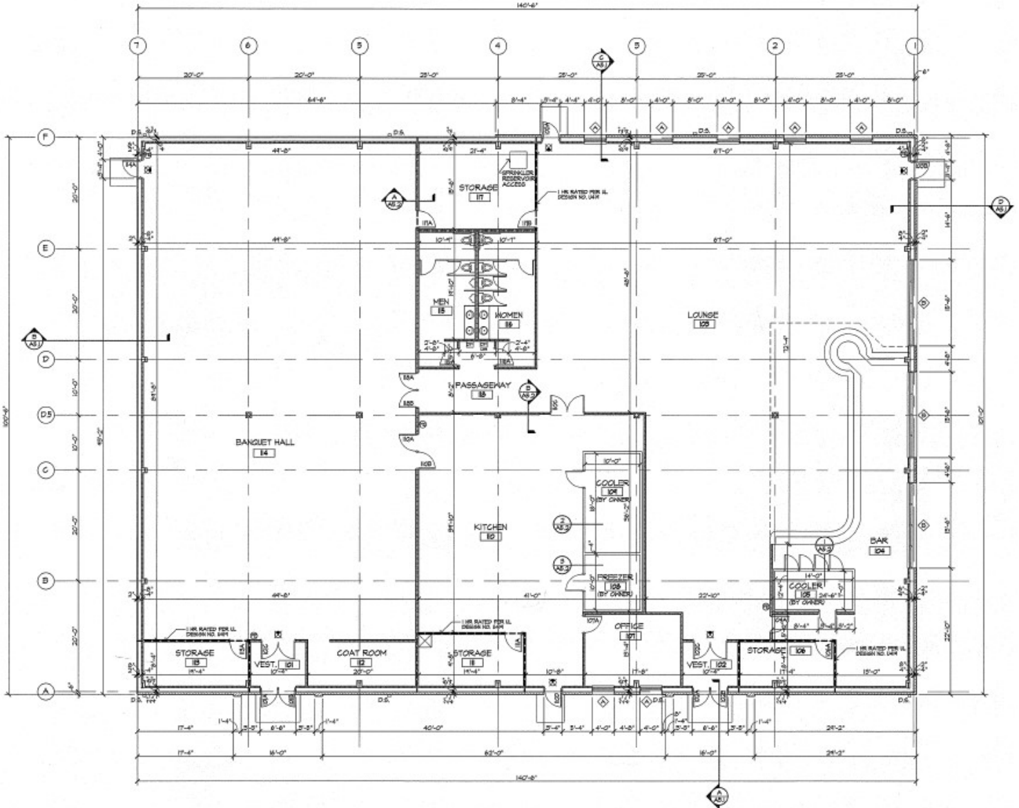
FLOOR PLAN 1/8" = 1'-0"
