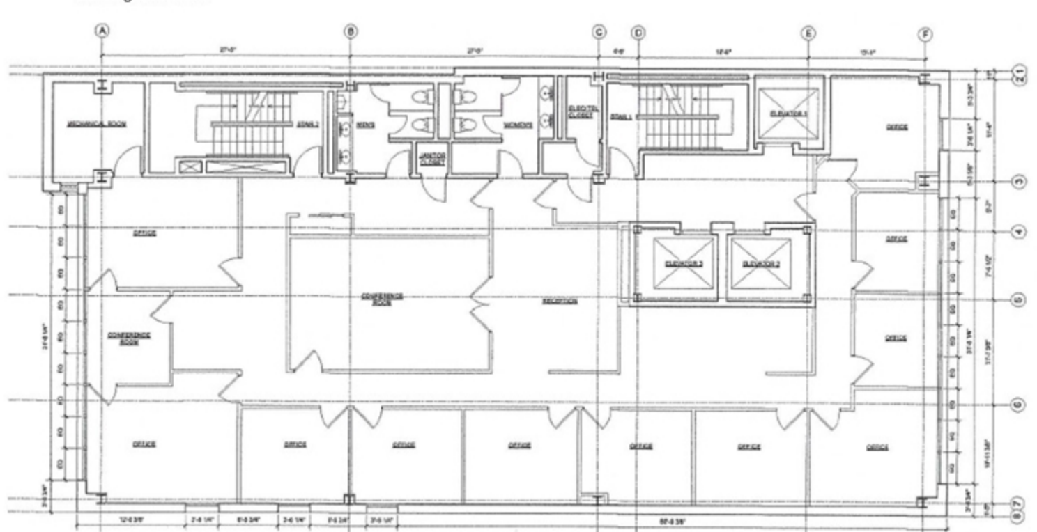
Entire 6 th Floor Plan Existing Conditions
