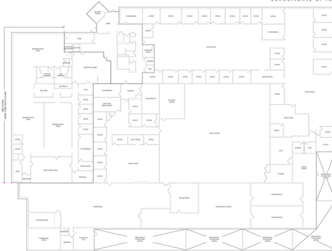
NORTH OVERALL SECOND FLOOR PLAN 1/16" = 1'-0"
