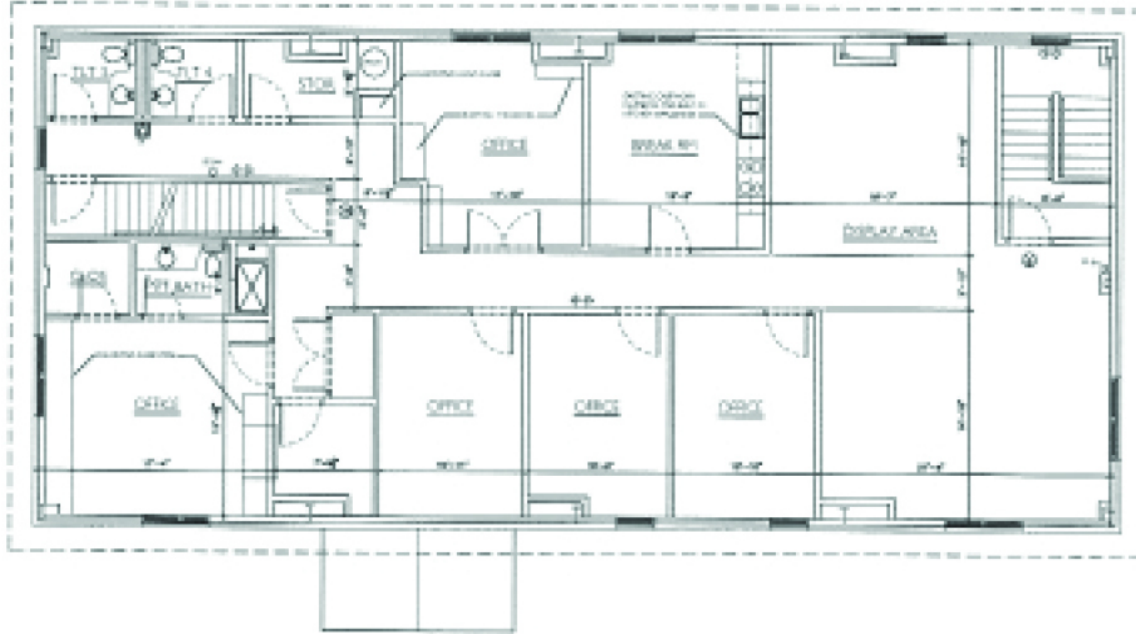
SECOND FLOOR
