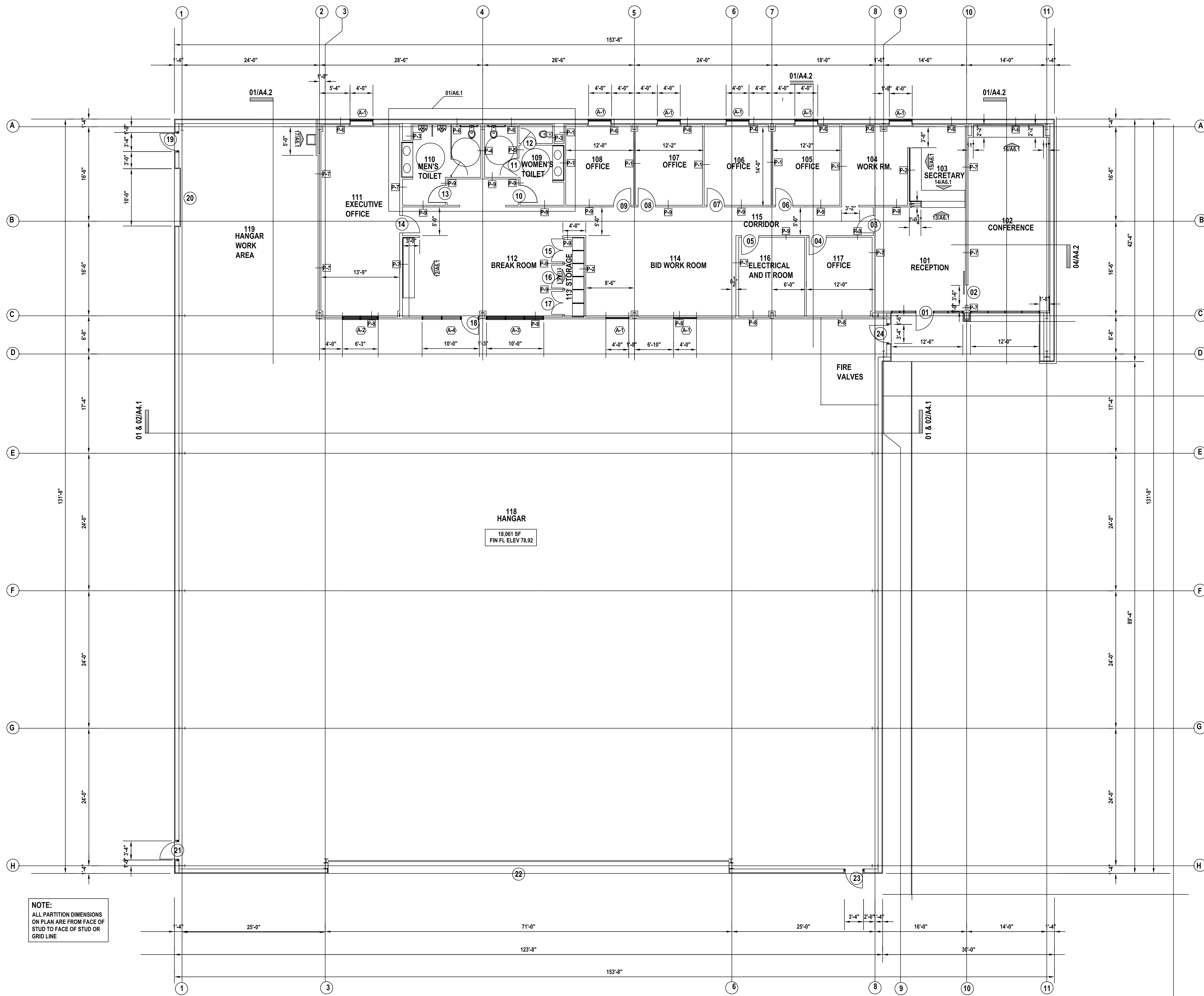
01 FLOOR PLAN SCALE: 1/8"=1'-0"
