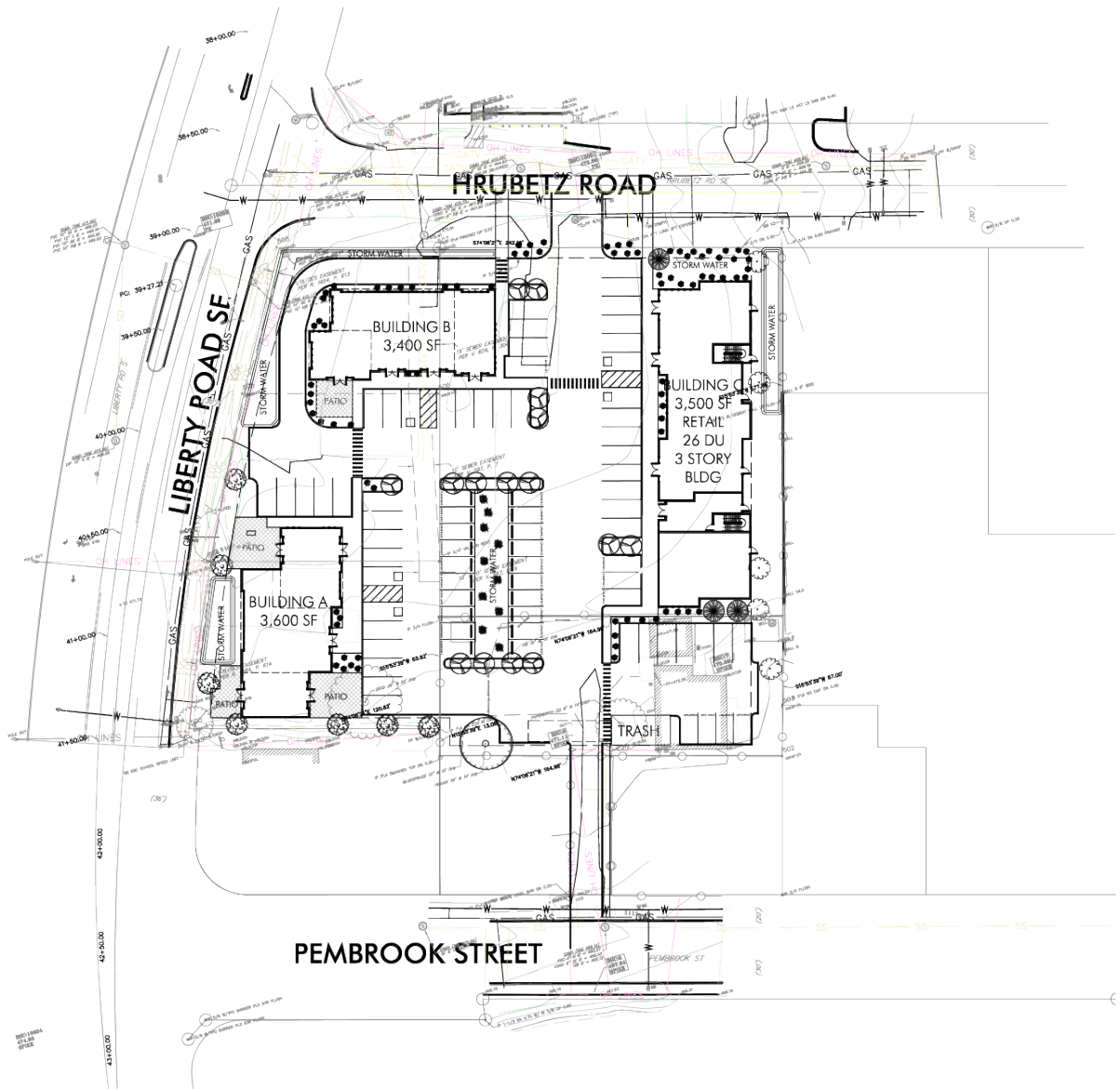
1 SITE PLAN 0 10' 20' 30' 40' 50' 60' 70' 80' 90' 100' 1:30
