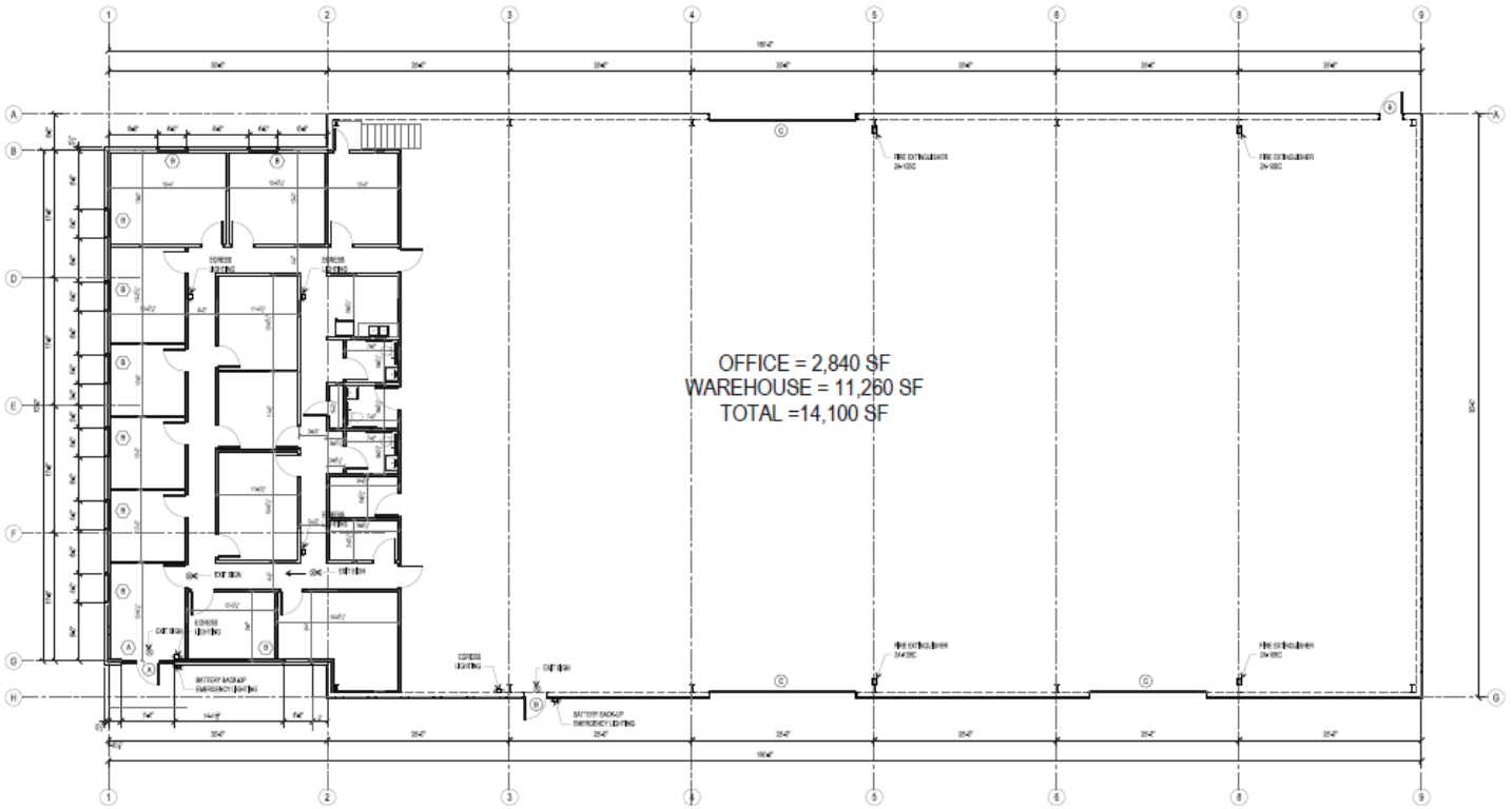
1 FLOOR PLAN 1/8" = 1'-0"
