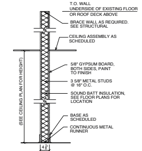
2 Partition Types A1.0 scale: 3/4" = 1'-0"
