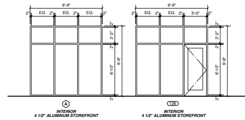
3 Storefront Elevation, Typical A1.0 scale: 1/2" = 1'-0"
