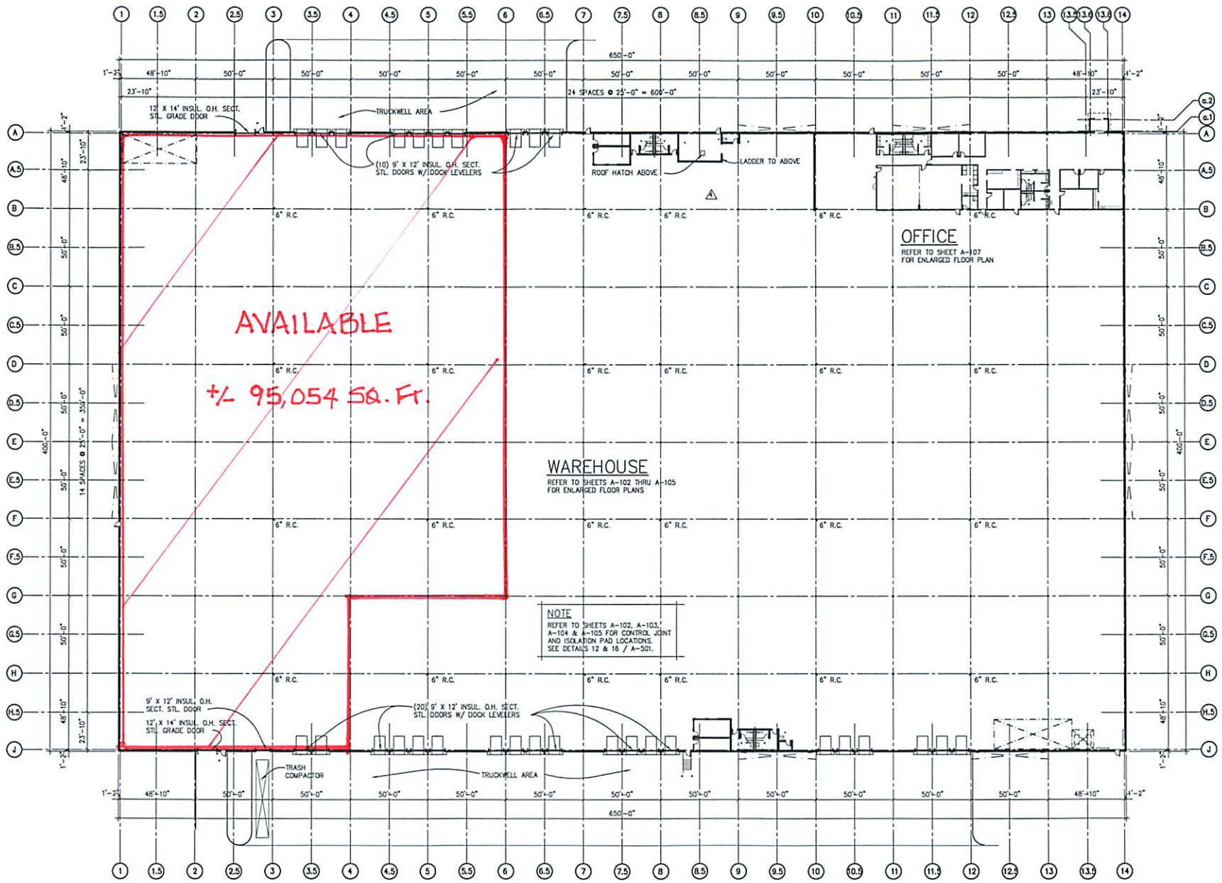
OVERALL FLOOR PLAN SCALE: 1/32" = 1'-0"
