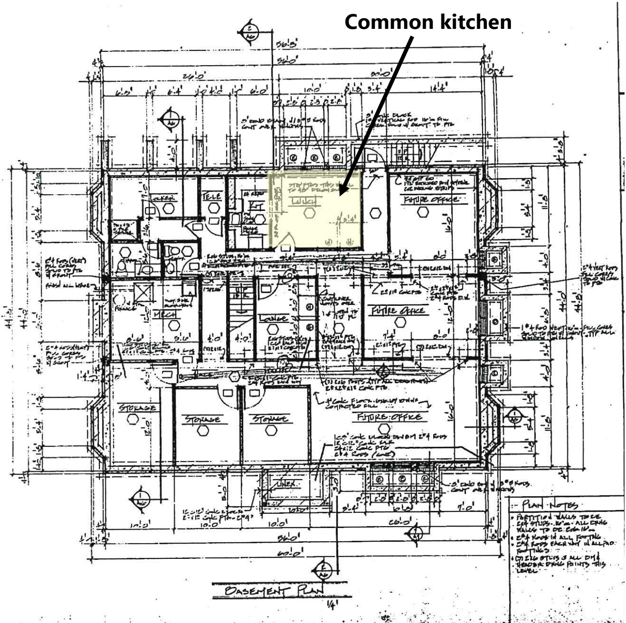
Lower level floor plan
