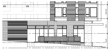
NE 50TH SIDEWALK ELEVATION
