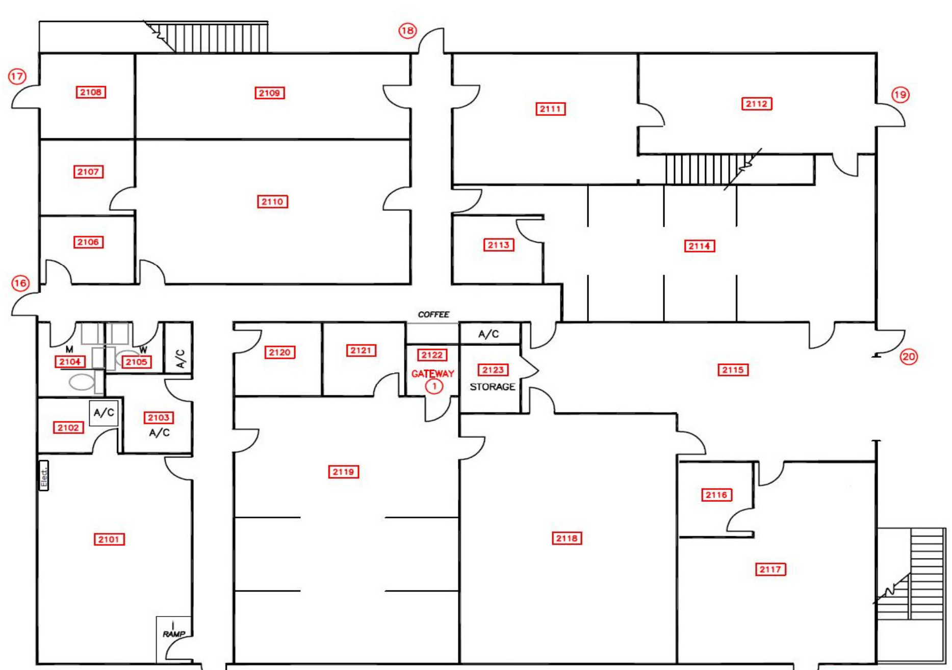
BUILDING 2 FIRST FLOOR (8000 Square feet) Scale in Feet
