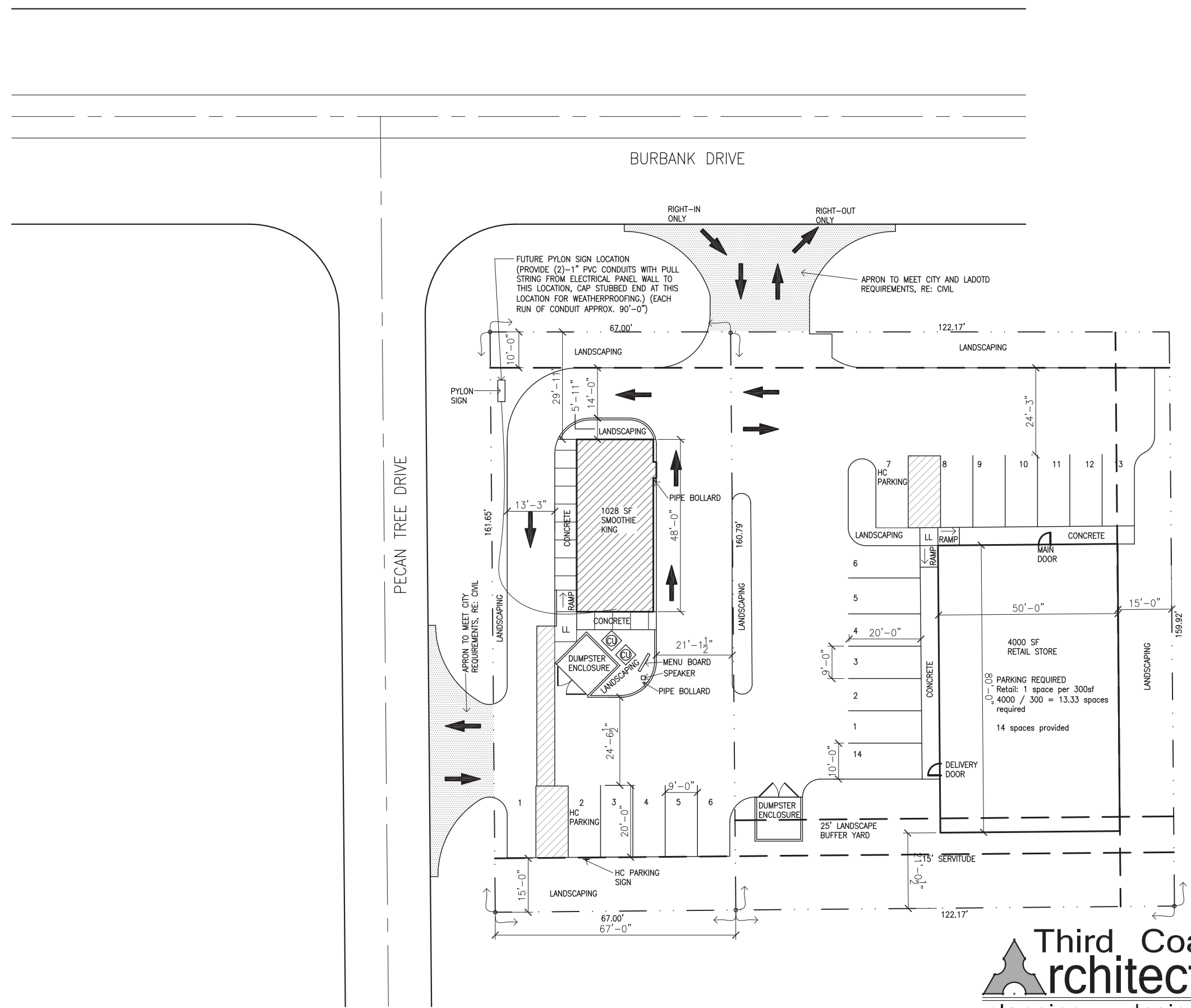
1 PROPOSED ARCHITECTURAL SITE PLAN SCALE: 1" = 30'-0"
