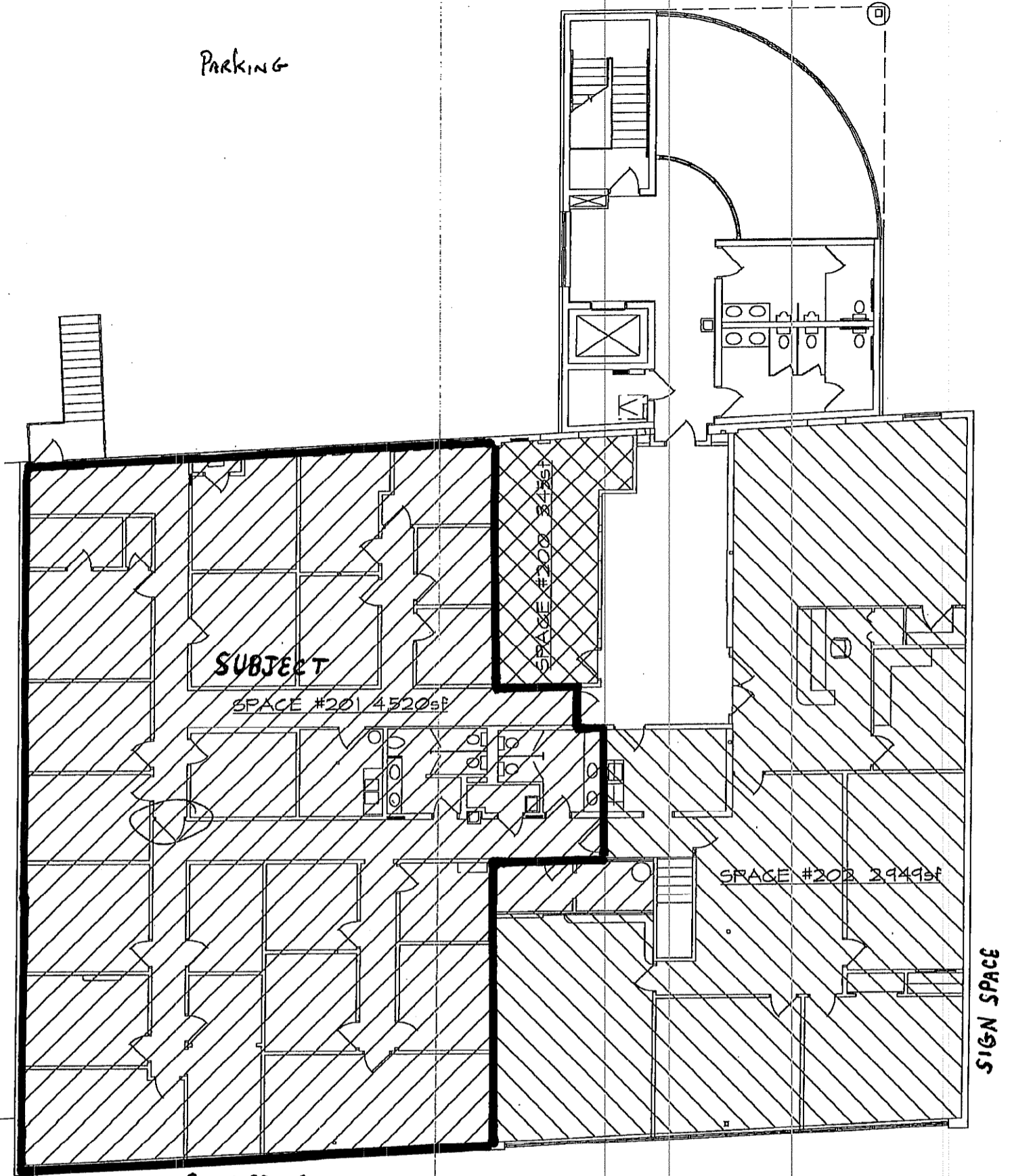
SIGN SPACE SECOND FLOOR PLAN
