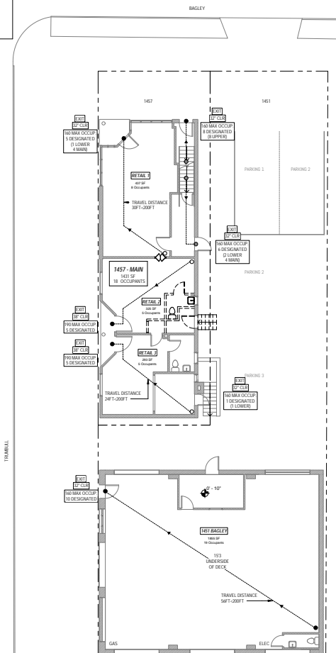
2 LIFE SAFETY PLAN - LEVEL 1
