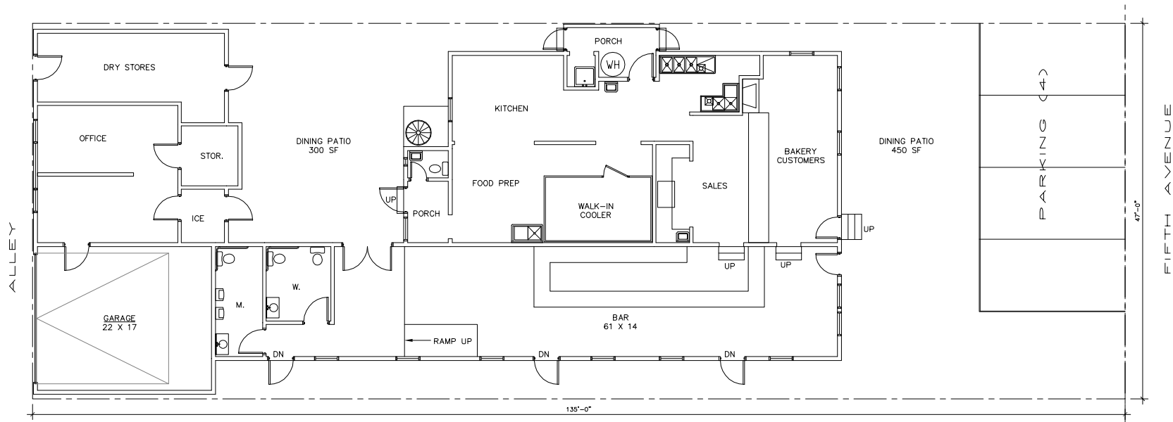
3766 FIFTH AVENUE - GROUND FLOOR AND SITE PLAN
