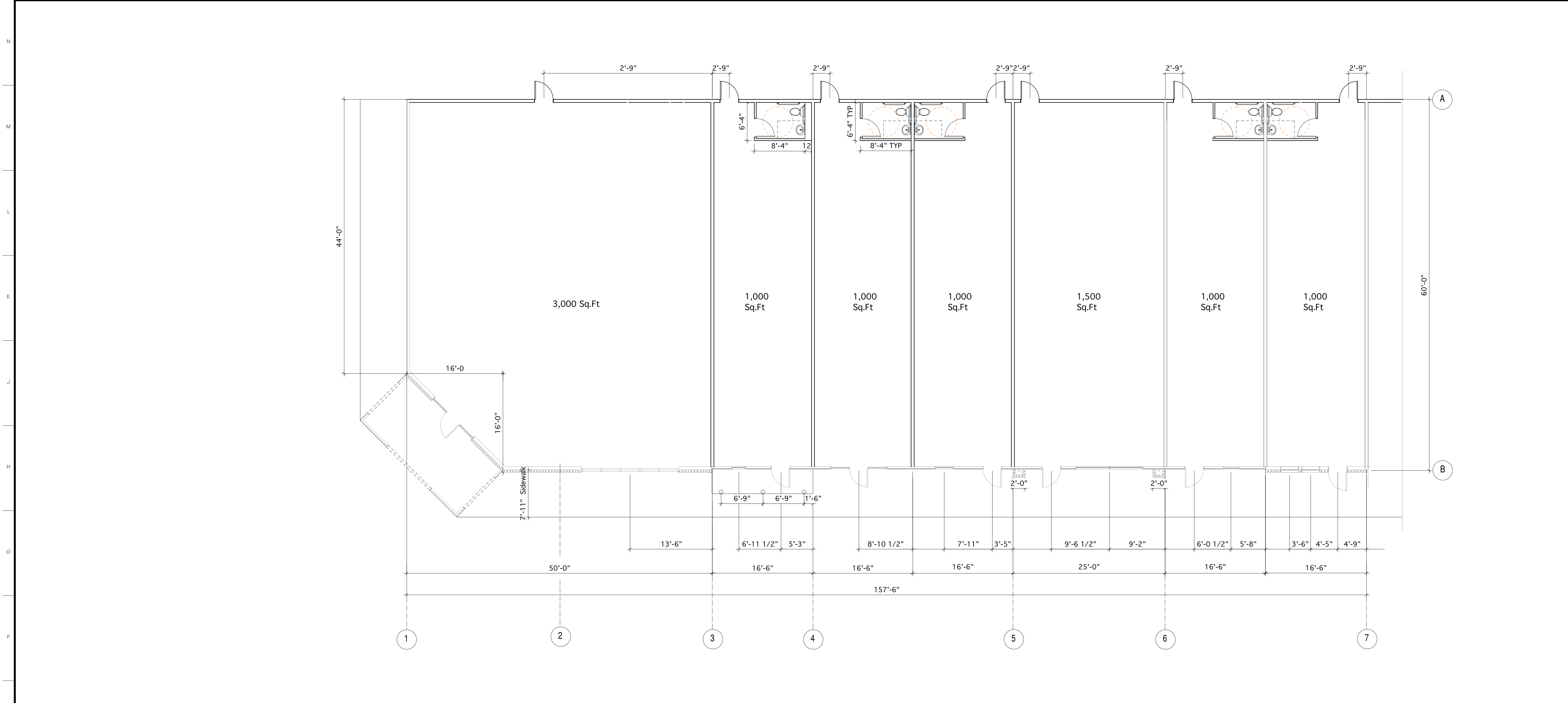
E.1 Partial Shell Plan Scale: 1/8" = 1'-0"
