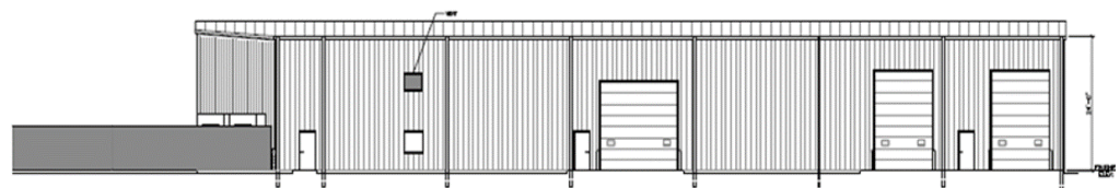
Building Elevation | East Elevation
