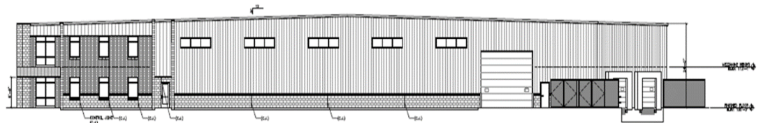
Building Elevation | South Elevation
