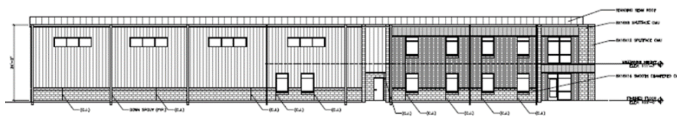
Building Elevation | West Elevation
