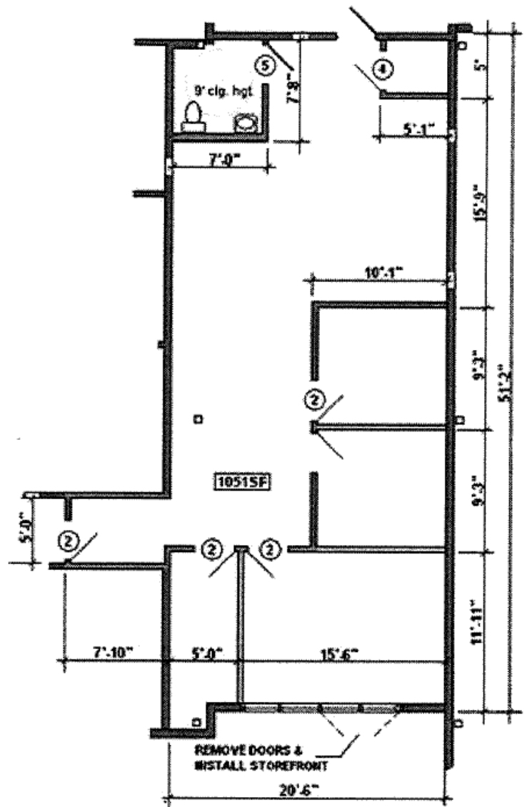
FLOOR PLAN (DIMENTIONED)
