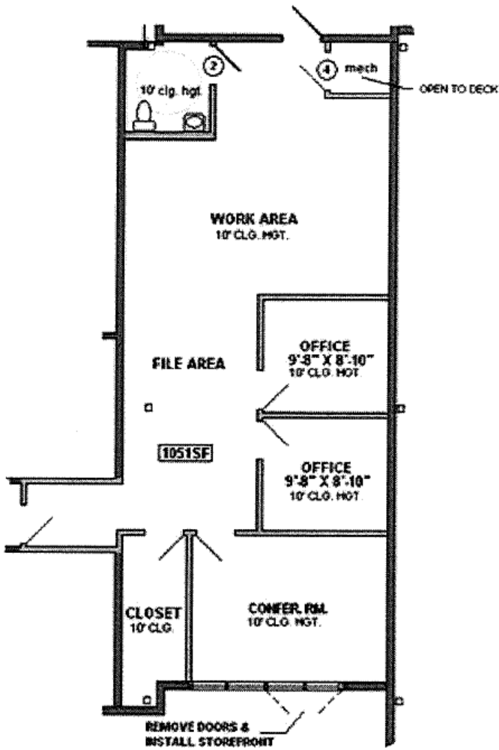
FLOOR LAY-OUT
